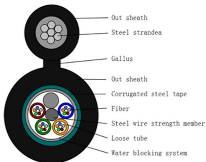
CABLE STRUCTURE AND PARAMETERS:
